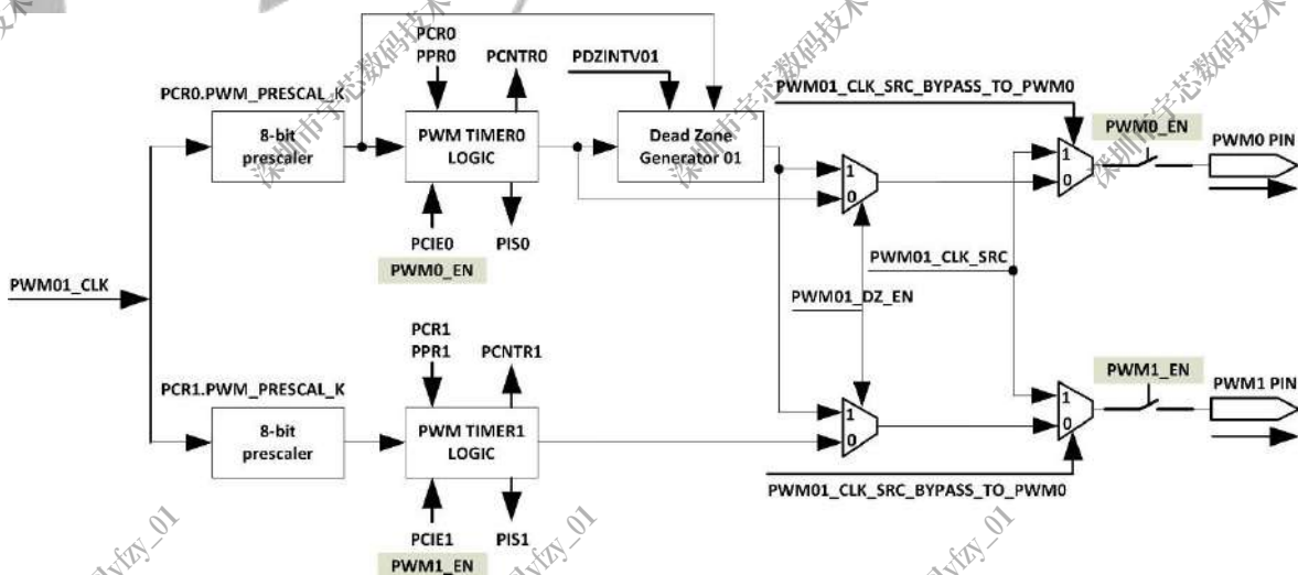
Figure 10-71 PWM01 Output Logic Module Diagram
