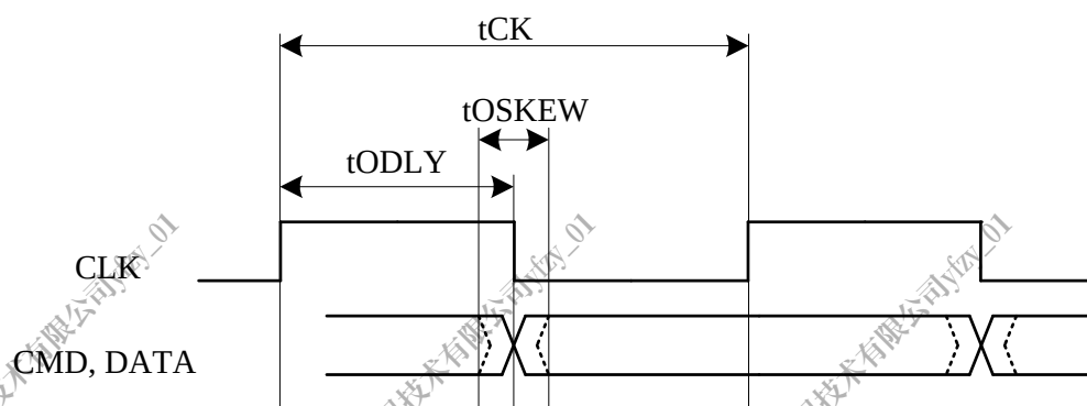
Figure 2-4 SMHC HS-SDR Mode Output Timing Diagram
