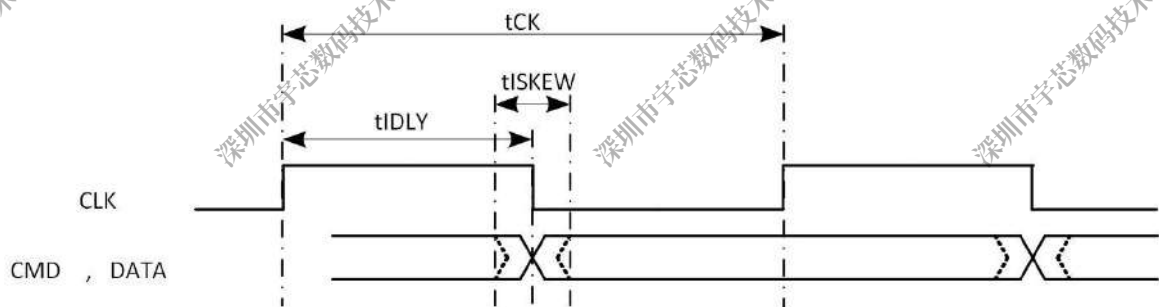
Figure 2-6 SMHC HS-SDR Mode Input Timing Diagram
