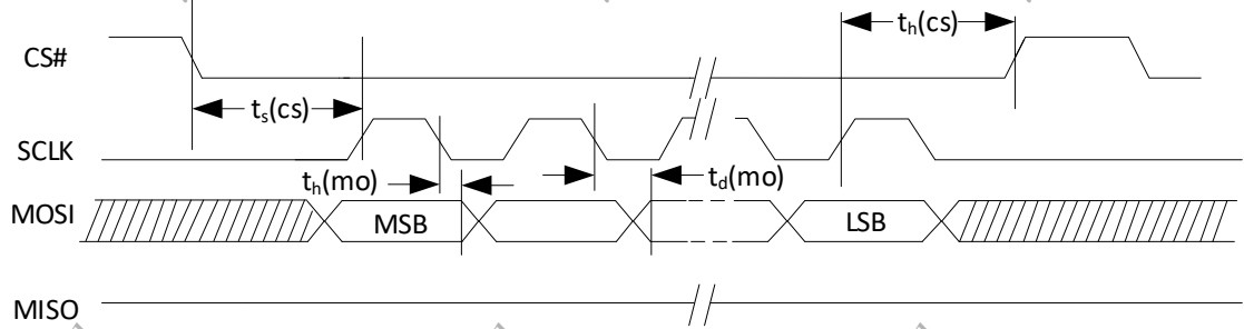
Figure 2-21 SPI MISO Timing
