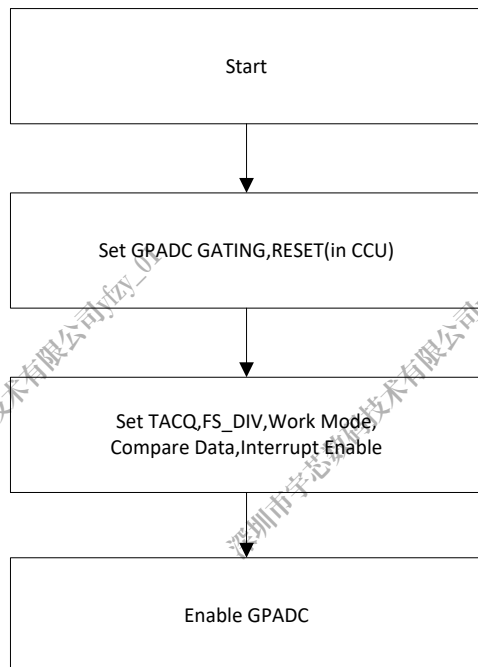
Figure 10-67 GPADC Initial Process
