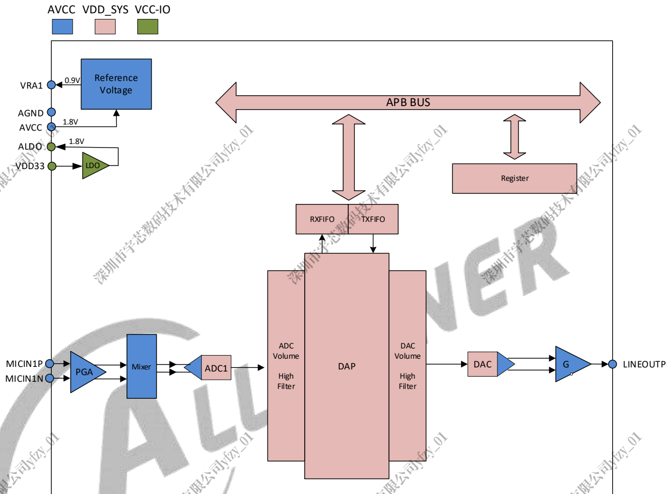
Figure 8-6 Audio Codec Block Diagram
