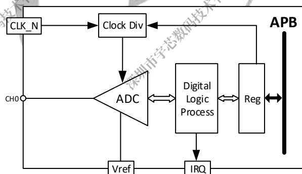
Figure 10-65 GPADC Block Diagram
