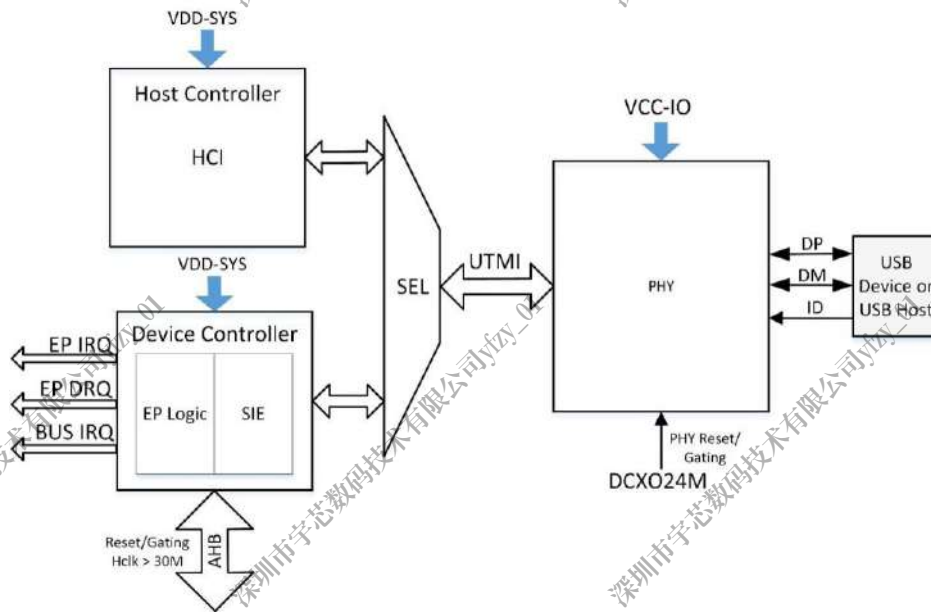
Figure 10-61 USB2.0 DRD Controller and PHY Connection Diagram
