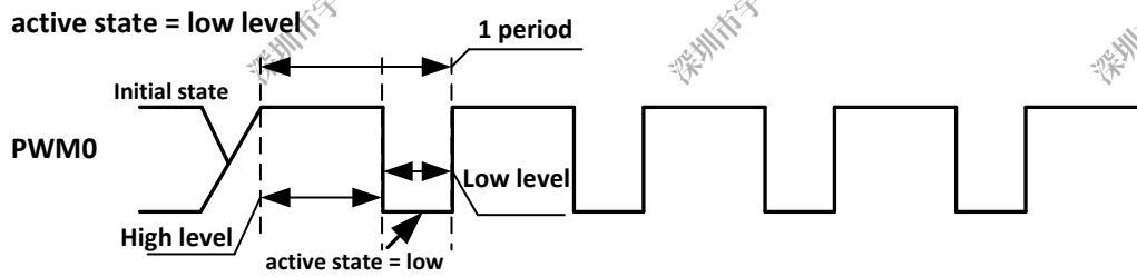
Figure 10-73 PWM0 Low Level Active State
