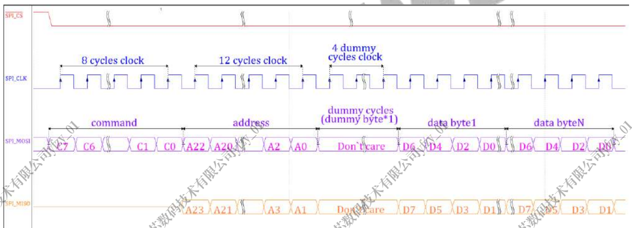
Figure 10-34 SPI Dual I/O Mode
