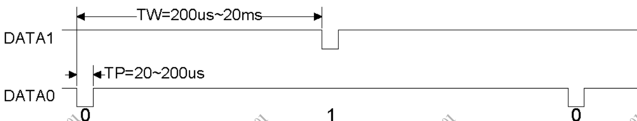
Figure 10-83 Data Signal Oscillogram
