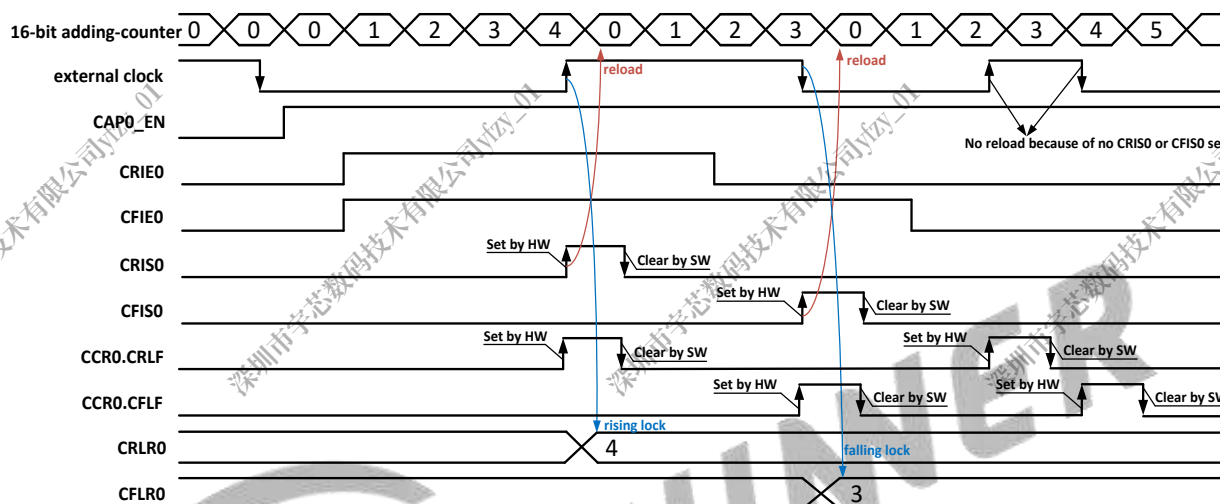
Figure 10-80 PWM0 Channel Capture Timing
