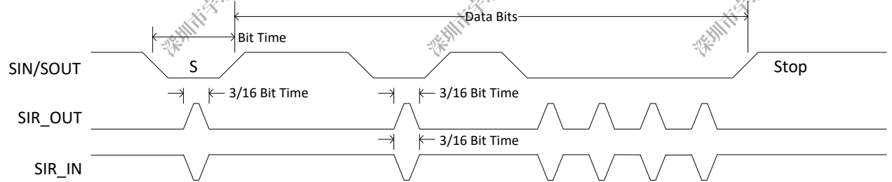
Figure 10-14 Serial IrDA Data Format
