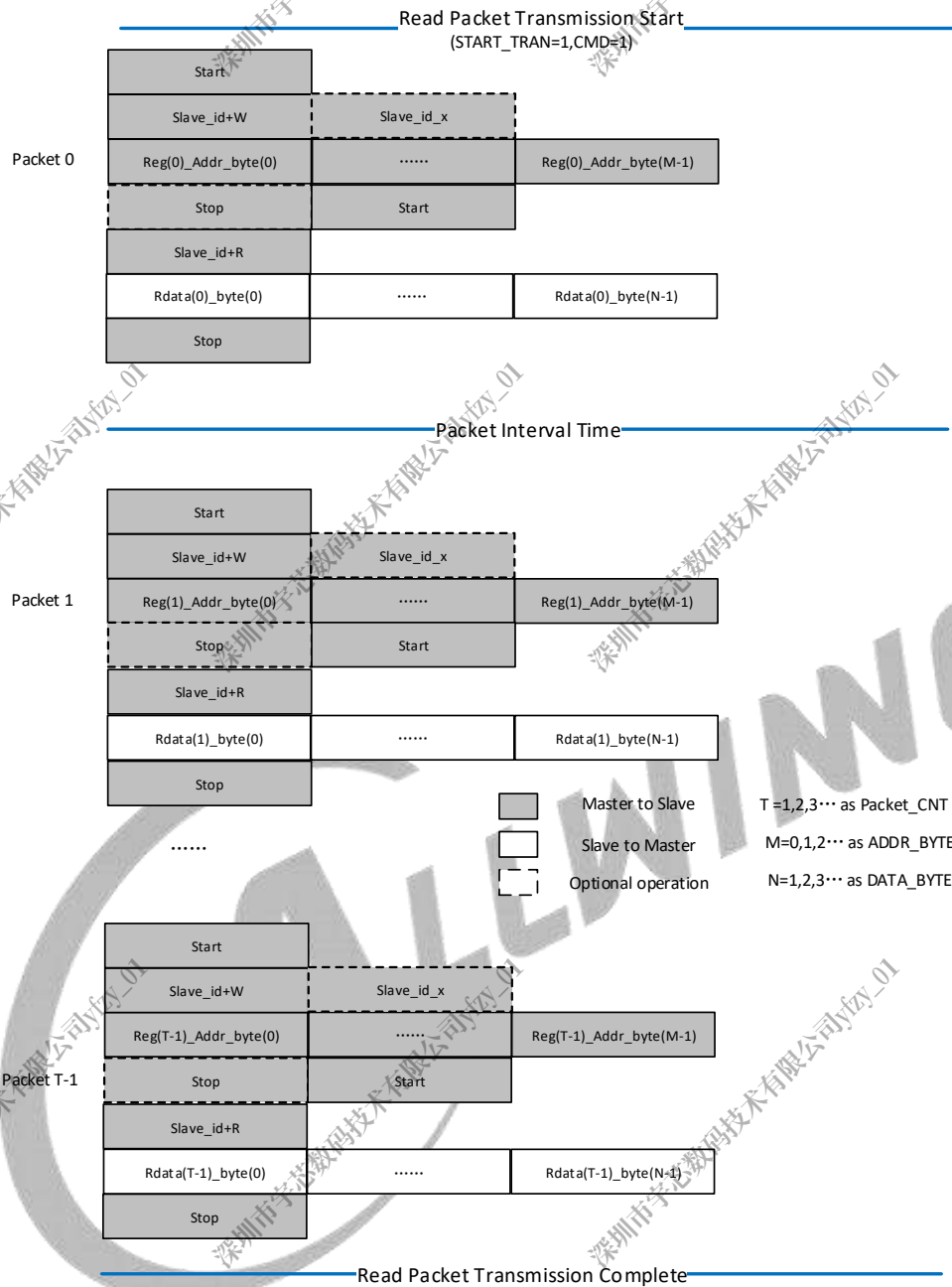
Figure 10-7 TWI Driver Read Packet Transmission
