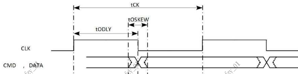
Figure 2-8 SMHC HS200 Mode Output Timing Diagram
