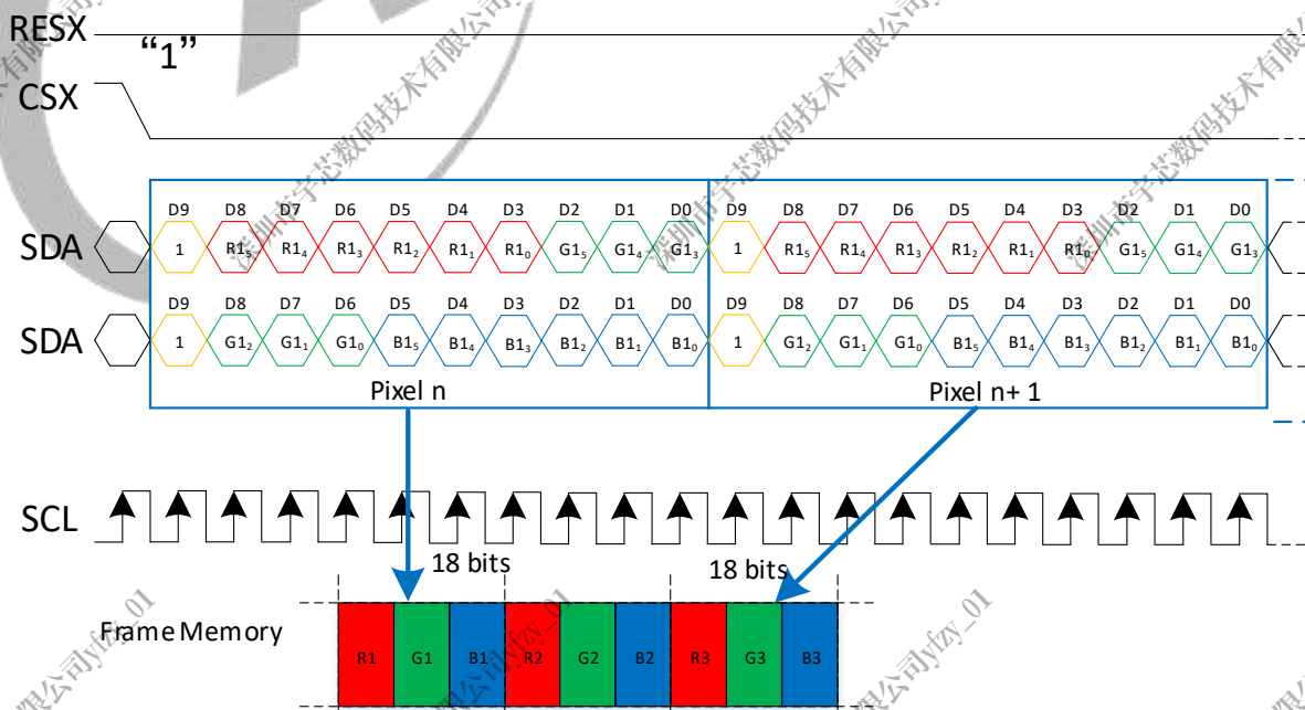
Figure 10-54 RGB666 2 Data Lane Interface Transmit Video Format 0
