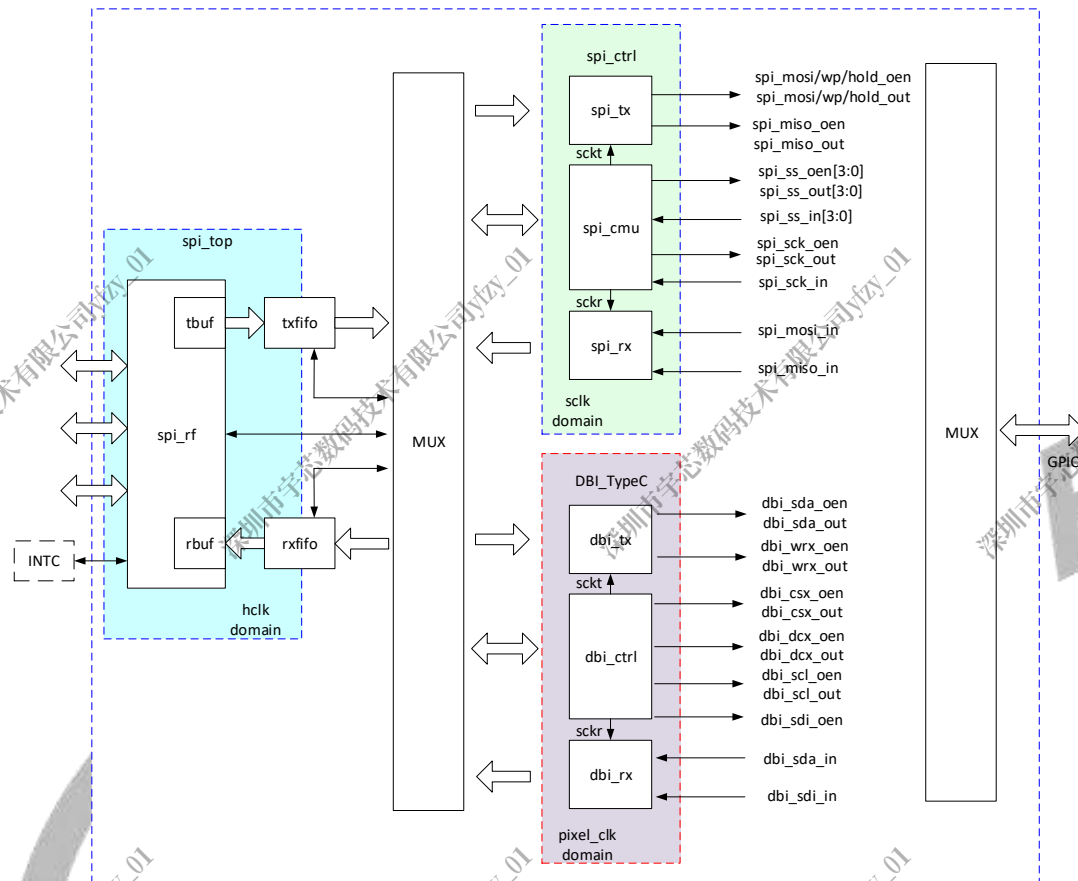
Figure 10-27 SPI_DBI Block Diagram
