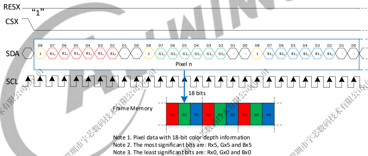
Figure 10-47 RGB666 3-Line Interface Transmit Video Format
