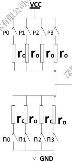
Figure 10-64 IO Buffer Strength Diagram
