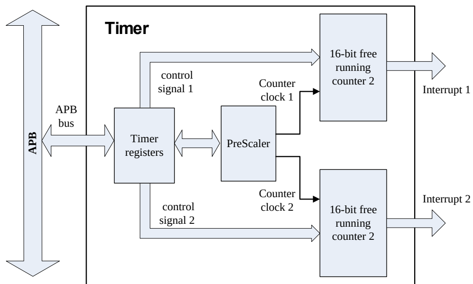
Figure 12-1 Timer Block Diagram
