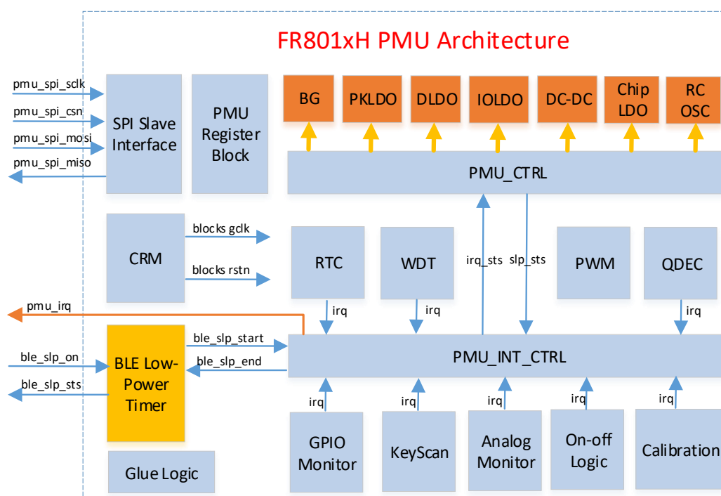
Figure 3-1 FR801xH PMU Architecture
